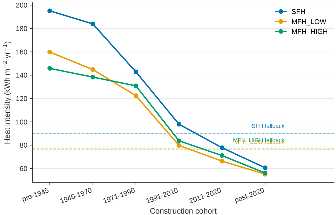
Heat intensity vs construction vintage, by building class
