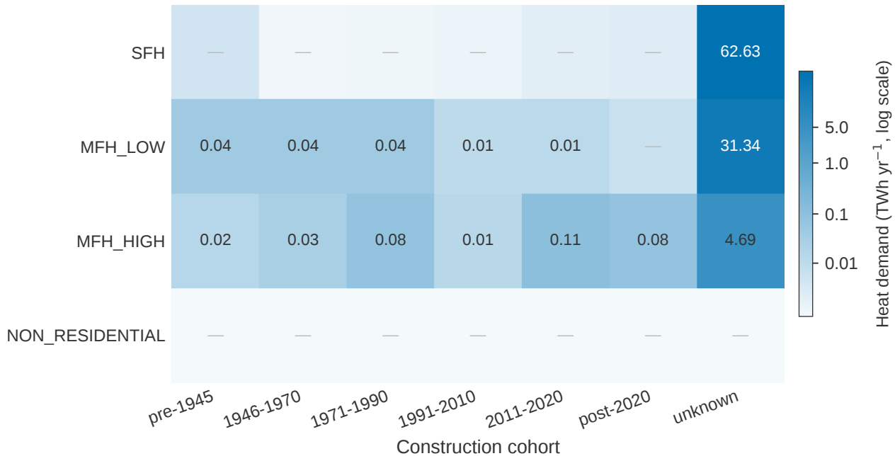
Heat demand by building class × construction cohort
