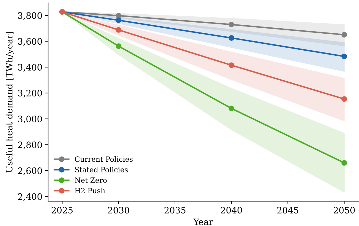
EU+CH+UK residential useful heat demand
