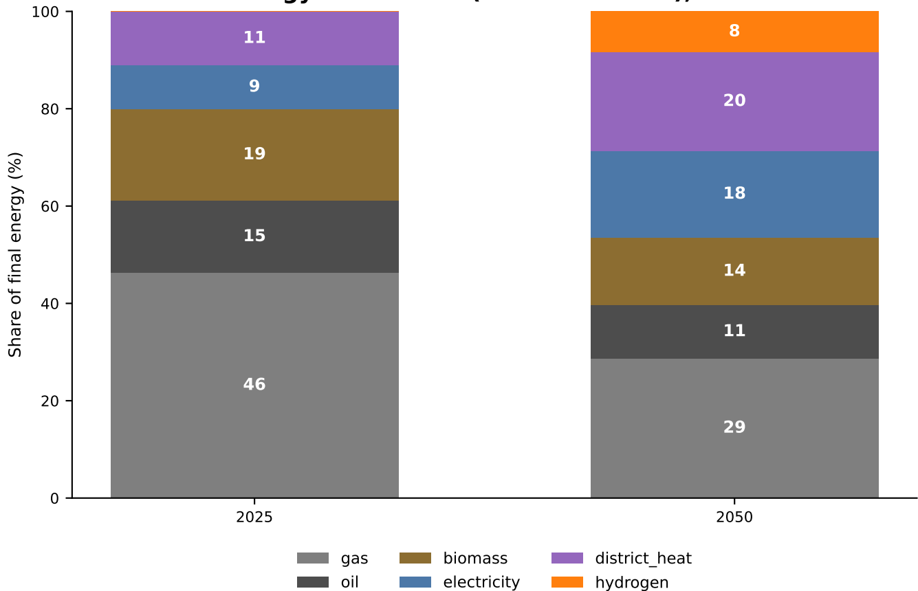
Final-energy carrier mix (Stated Policies), 2025-2050
