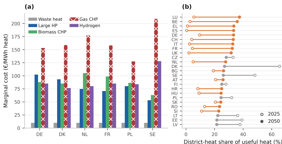
Figure A.9: District heating. Panel (a) is the merit-order stack under H2 Push, the scenario most favourable to hydrogen; panel (b) is the Net Zero build-out. The two panels are on different scenarios deliberately, so the stack is read at hydrogen’s best and the expansion at the deepest decarbonisation.
