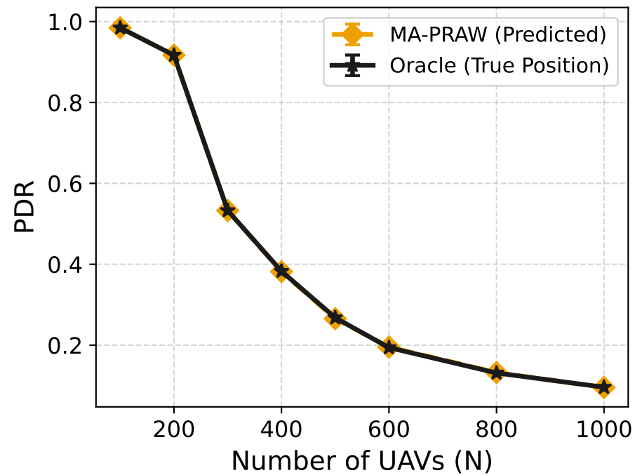
Cluster-based PDR
