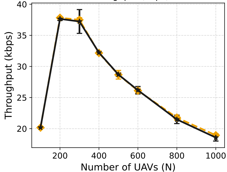
Throughput (kbps)
