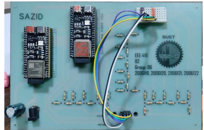
Hardware Implementation
