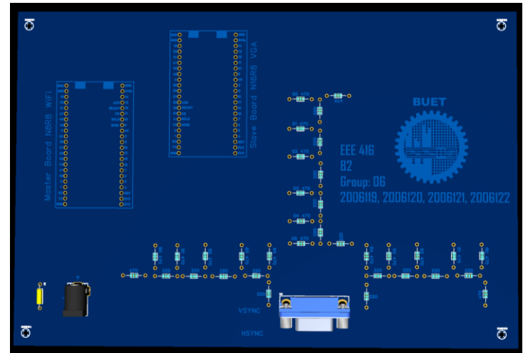
PCB Design
