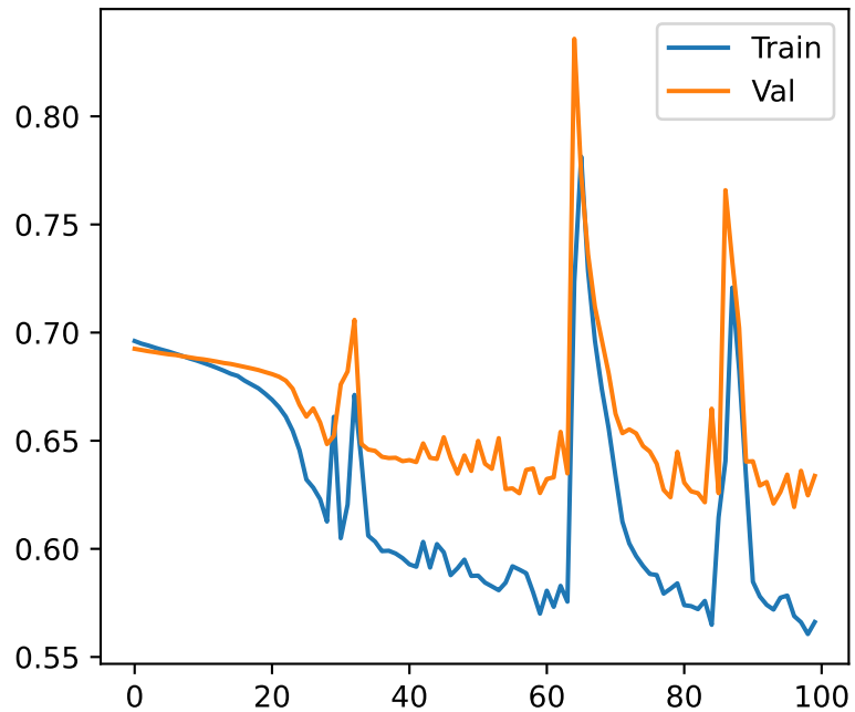
Loss e=100 l=1 h=32
