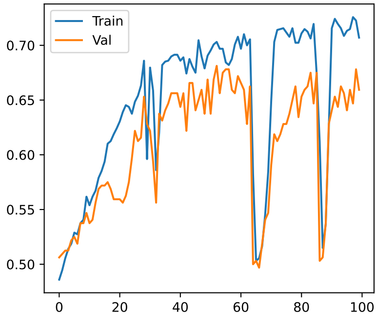
Accuracy
