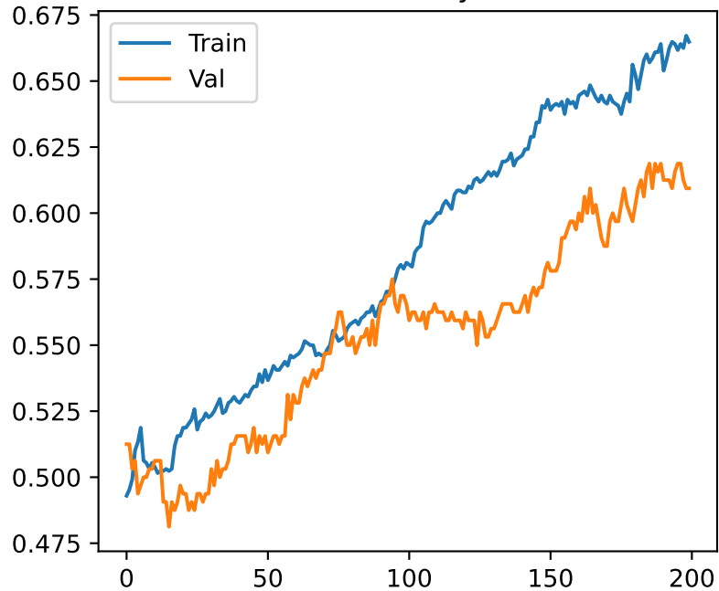
Accuracy
