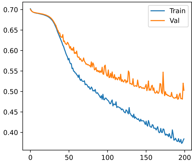
Loss e=200 l=2 h=16
