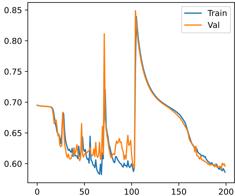
Loss e=200 l=5 h=16
