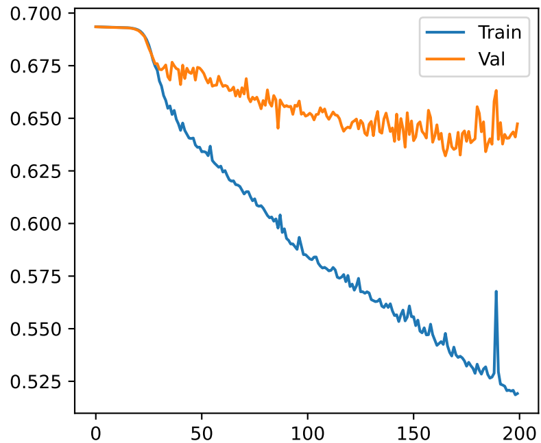
Loss e=200 l=5 h=8
