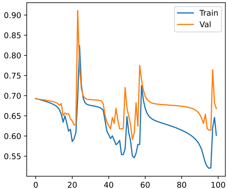
Loss e=100 l=1 h=64
