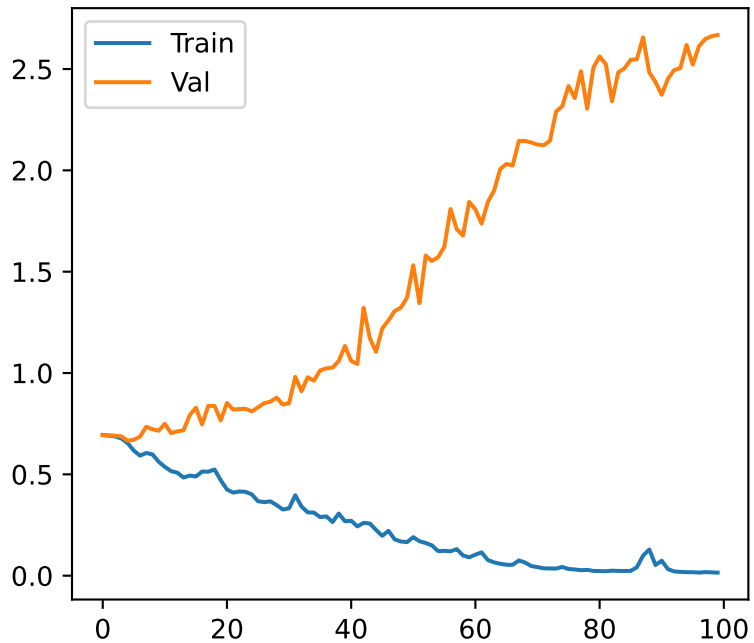
Loss e=100 l=3 h=128
