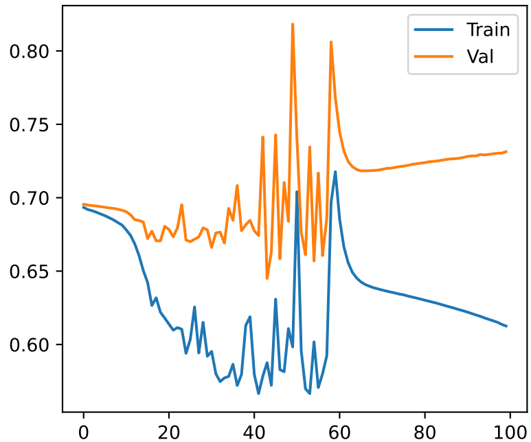
Loss e=100 l=3 h=32
