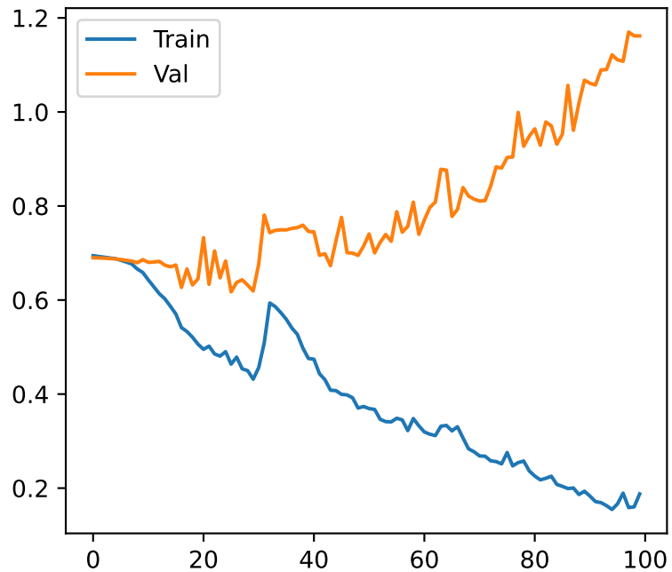
Loss e=100 l=3 h=64
