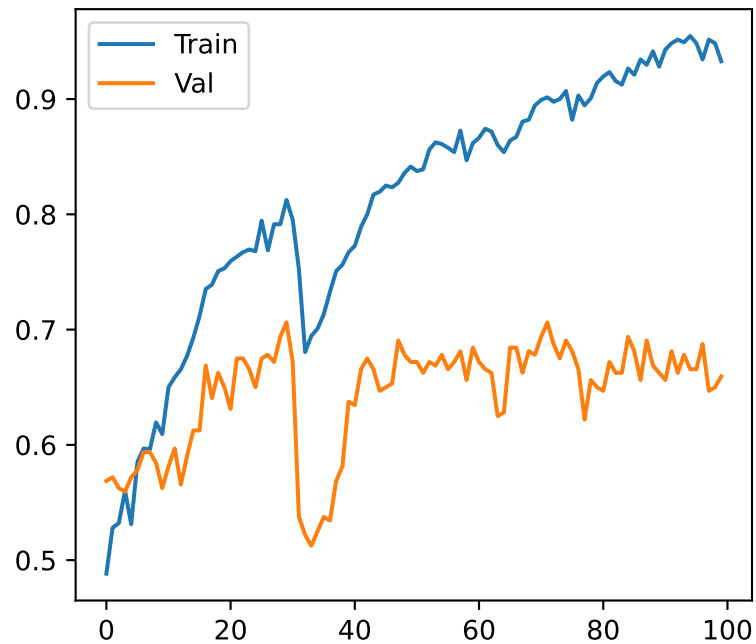
Accuracy
