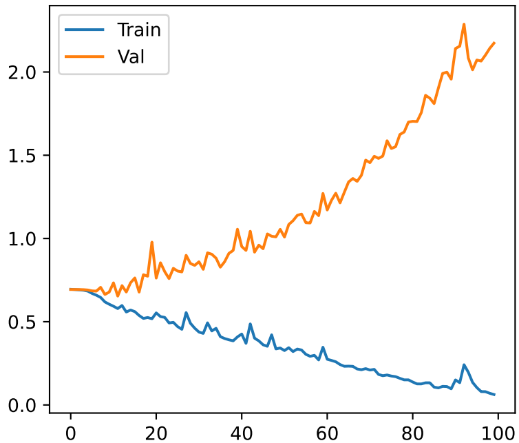
Loss e=100 l=5 h=64
