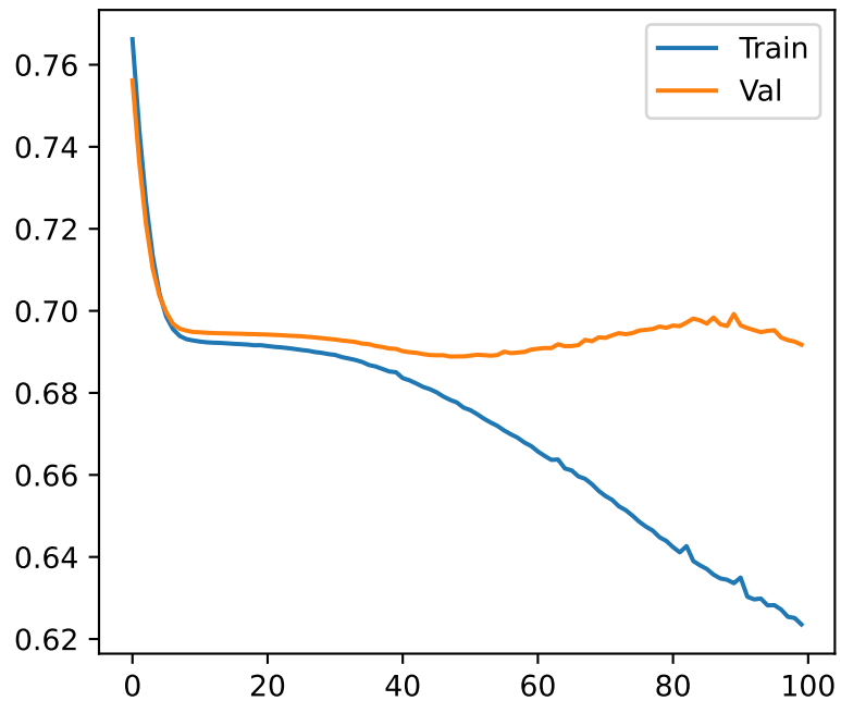
Loss e=100 l=5 h=8
