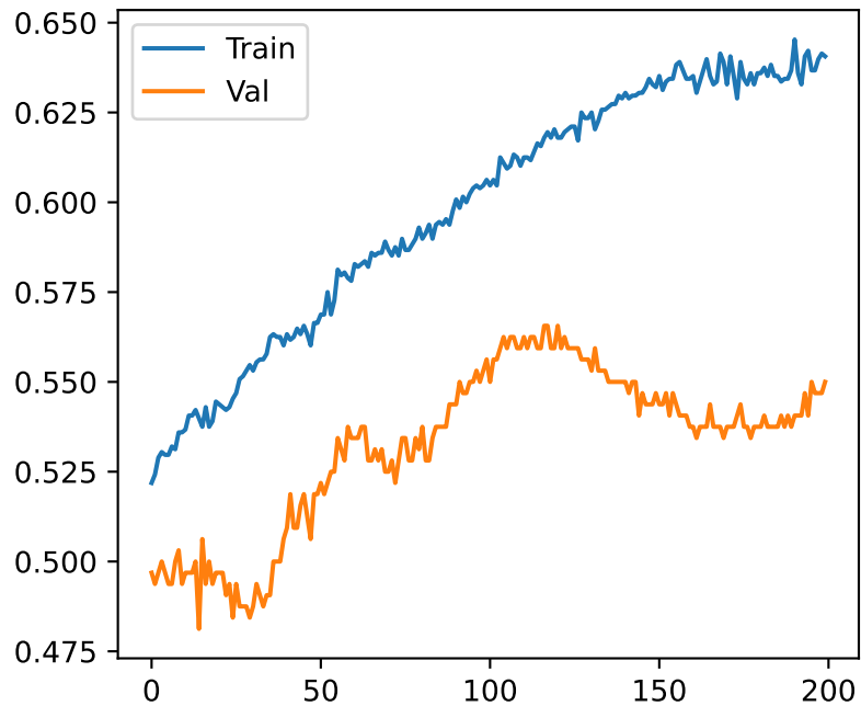
Accuracy
