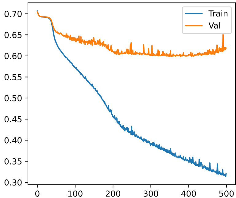
gru model - Layers: 5, Hidden Dim: 8, LR: 0.0001 Loss Accuracy
