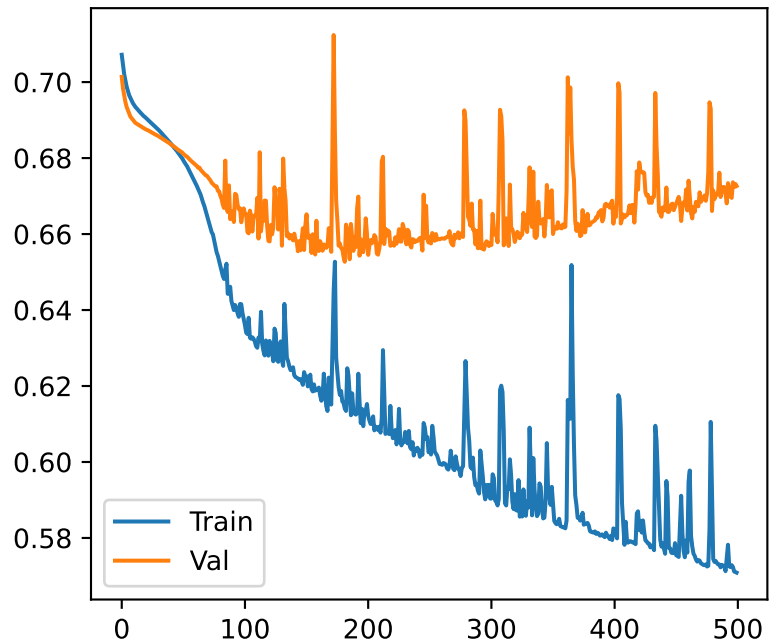
rnn model - Layers: 1, Hidden Dim: 8, LR: 0.0001 Loss Accuracy
