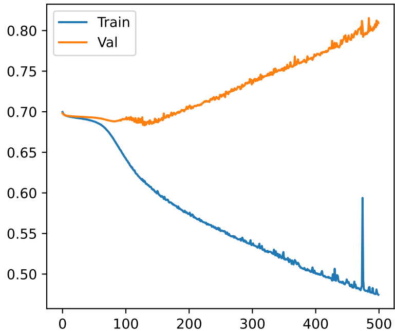
rnn model - Layers: 3, Hidden Dim: 8, LR: 0.0001 Loss Accuracy
