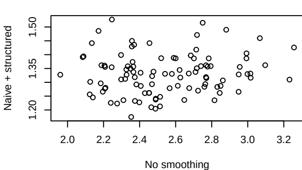
AIS (per simulation)
