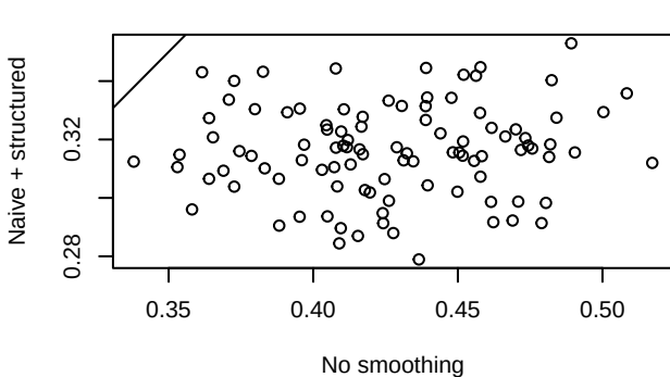
RMSE (per simulation)
