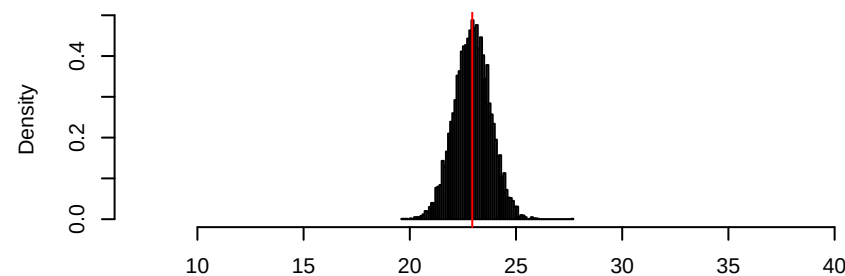
Bootstrap Distribution
