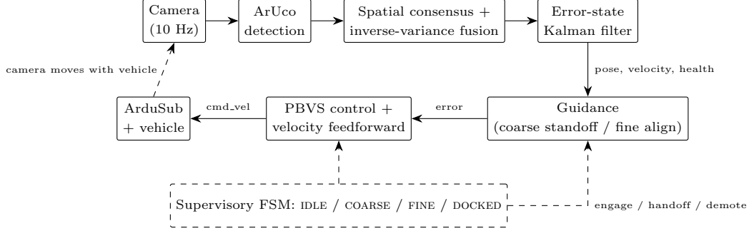
Figure 9: System architecture. The state machine gates the controllers on the filter’s health signal, and the vehicle-to-camera feedback path is the ego-motion coupling analysed in Section 4.1.
