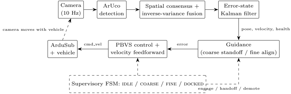
Figure 1: System architecture. Perception runs entirely in the loop; the supervisory state machine sequences the mission and gates the controllers on the filter’s health signal. The feedback path from vehicle to camera is the ego-motion coupling analysed in Section 4.1.
