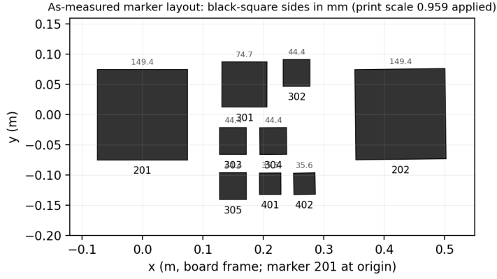
Figure 5: As-measured marker layout in the board frame, positions and black-square sides estimated from the data with the 0.959 print scale applied. The four size groups placed at a common range are the marker-size lever of the experiment.
