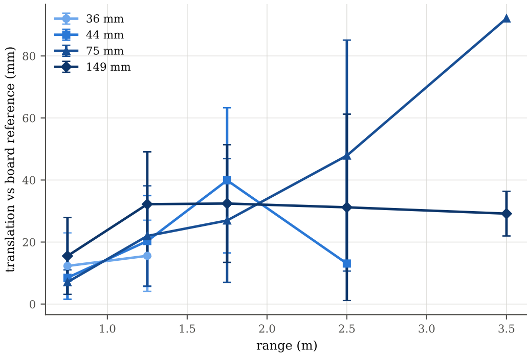
Single-marker vs board reference (self-consistency, NOT accuracy)
