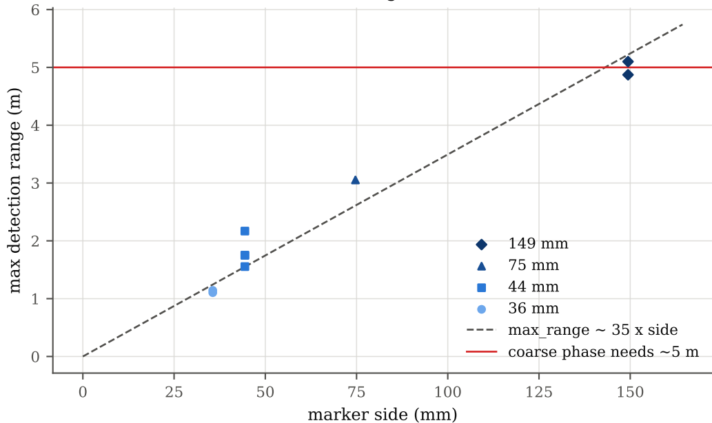
Max detection range vs marker size
