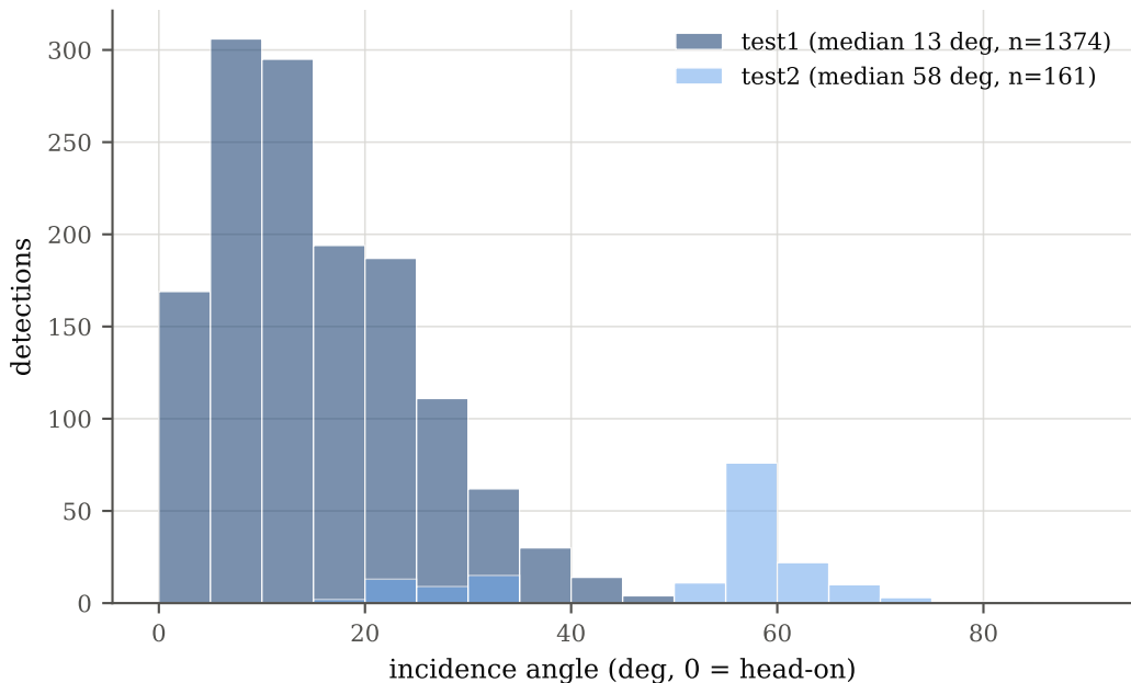
Incidence angle: two regimes, no sweep angle was never controlled and is confounded with range and marker size
