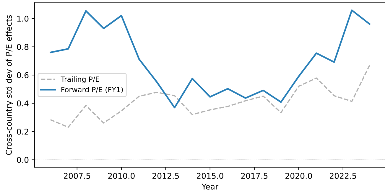
P/E Dispersion: Forward vs Trailing (both with R&D + LTG controls)
