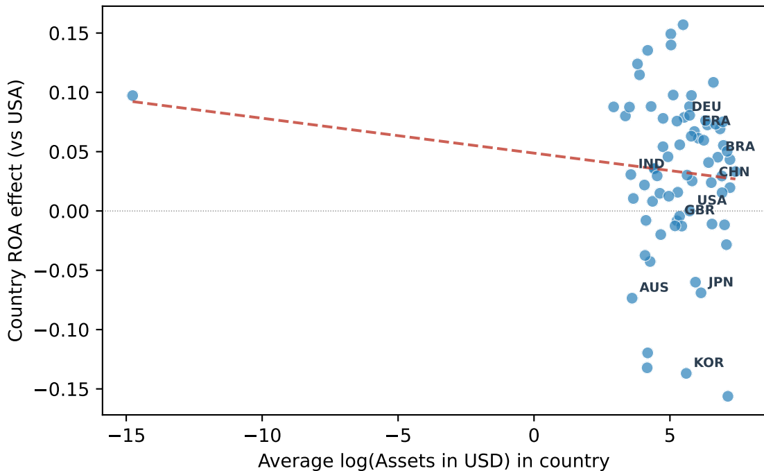
Firm Size (USD) vs ROA Effect ( r = -0.12 )
