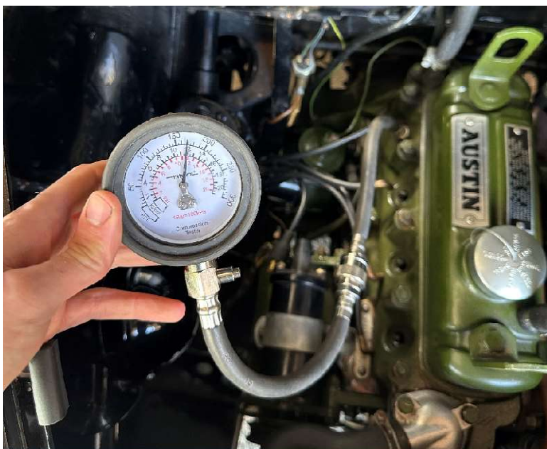
Cylinder 4 Compression test result
