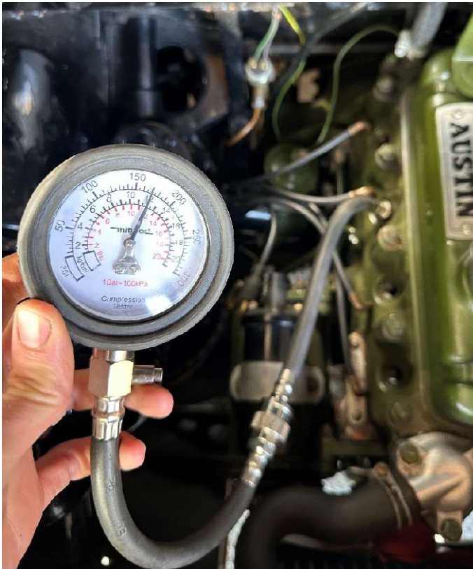
Cylinder 4 Compression test result
