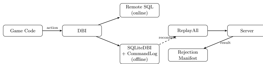
Figure 1: Hybrid persistence architecture: game code interacts only with the DBI; the active implementation is swapped at runtime depending on connectivity.
