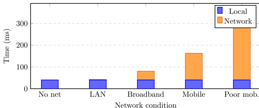
Figure 7: Reconnection time breakdown for 10,000 commands: local processing is constant at \sim 40 ms; network RTT dominates under high-latency conditions.
