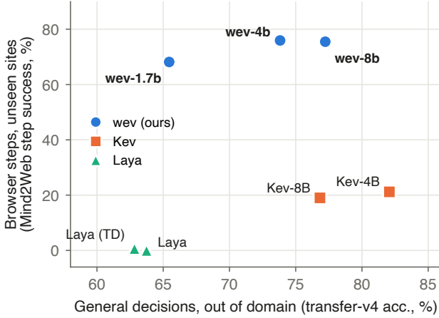
Figure 1. Browser steps against general decisions (test splits). Open decision models trained on general data stay below 22% step success on unseen websites; WEV reaches 68–76% while remaining competitive out of domain.
