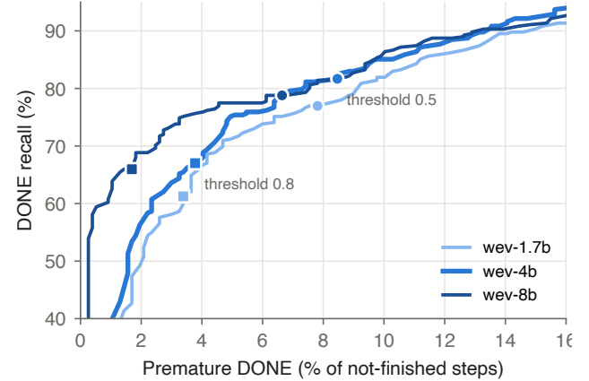
Figure 3. Stopping trade-off on the NNetNav test split (382 DONE steps, 768 others). Each curve accepts DONE only when its probability exceeds a threshold swept from 0.05 to 0.99; circles mark 0.5 and squares 0.8.
