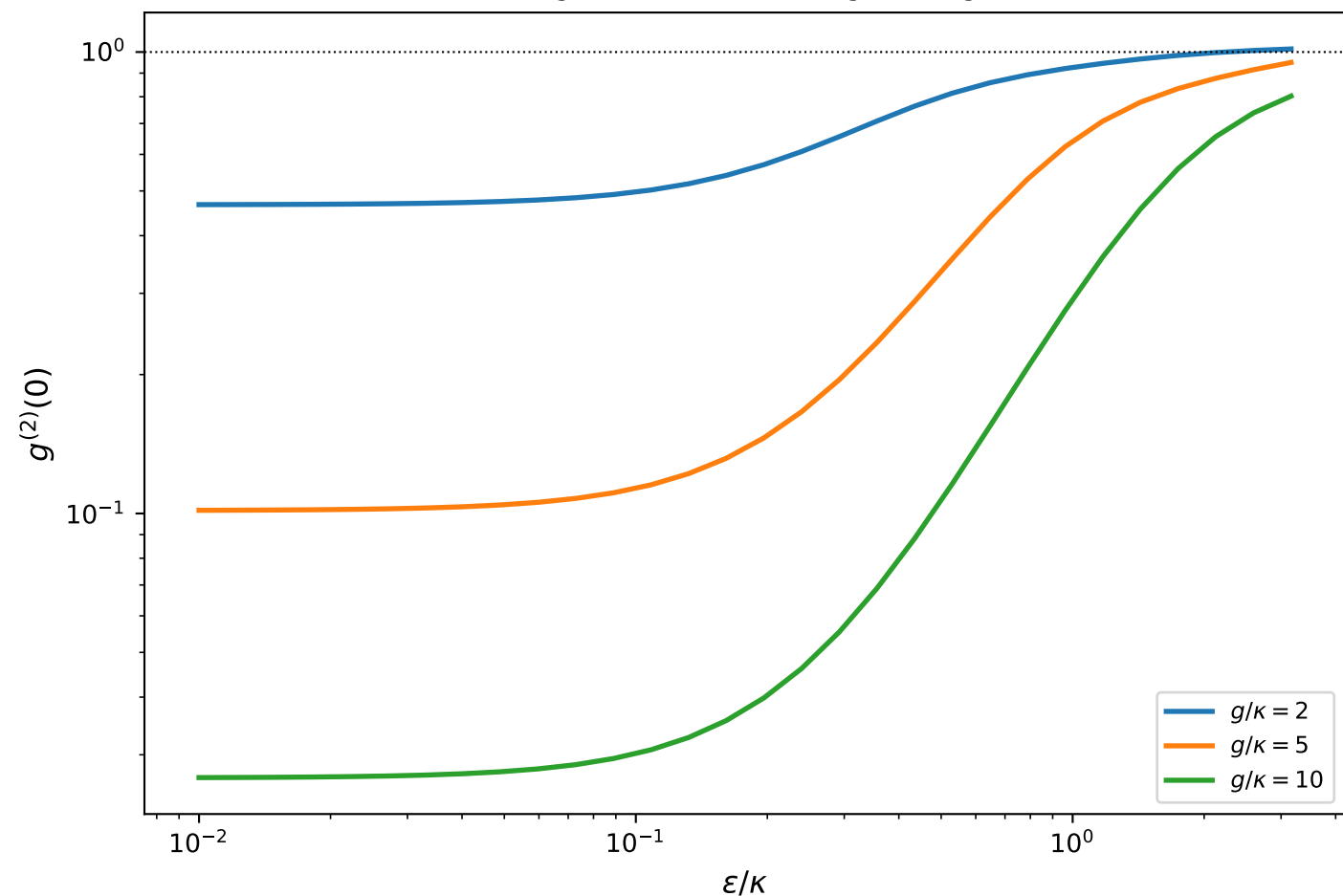
(b) g^{(2)}(0) vs drive strength, \Delta = g
