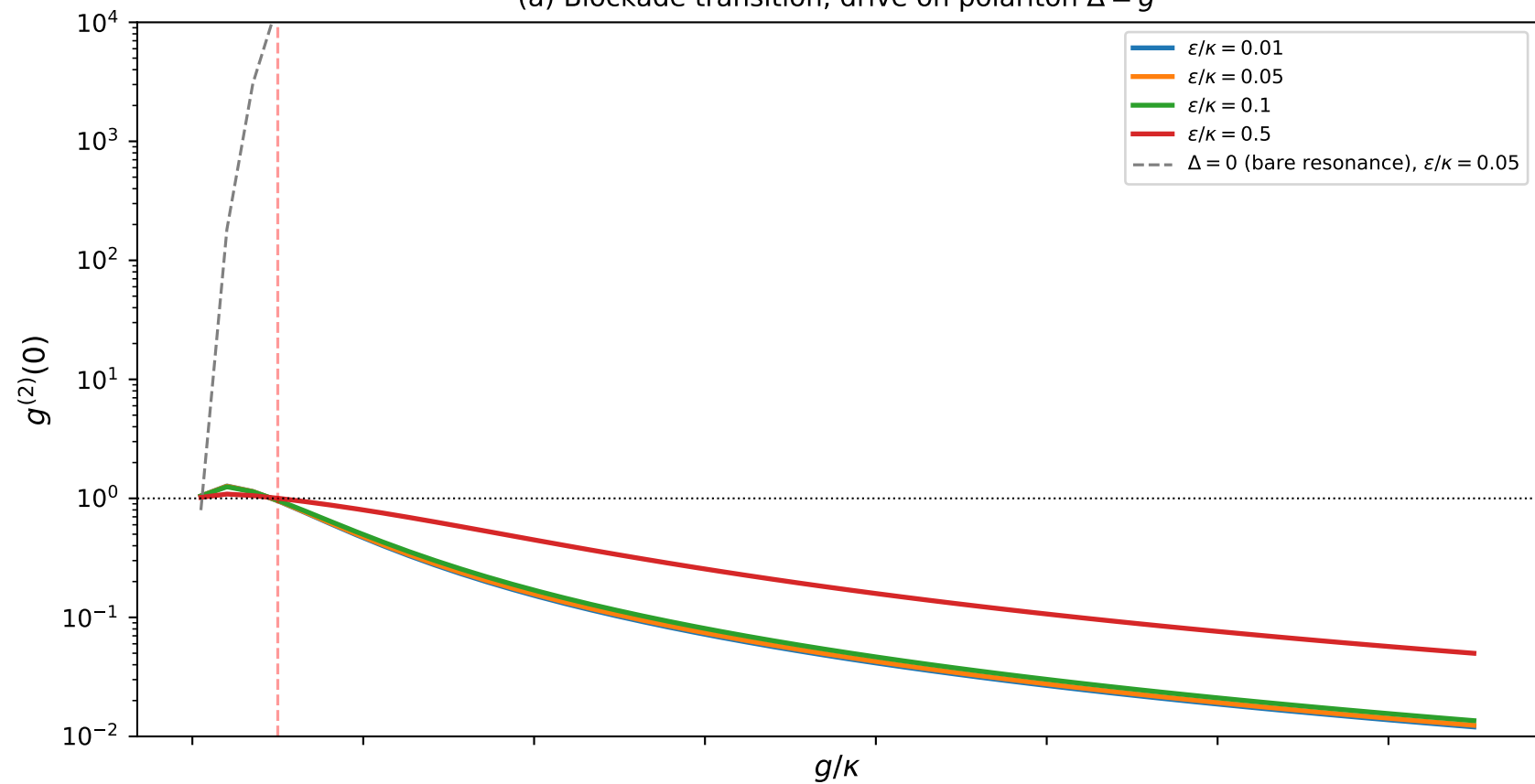
(a) Blockade transition, drive on polariton \Delta = g
