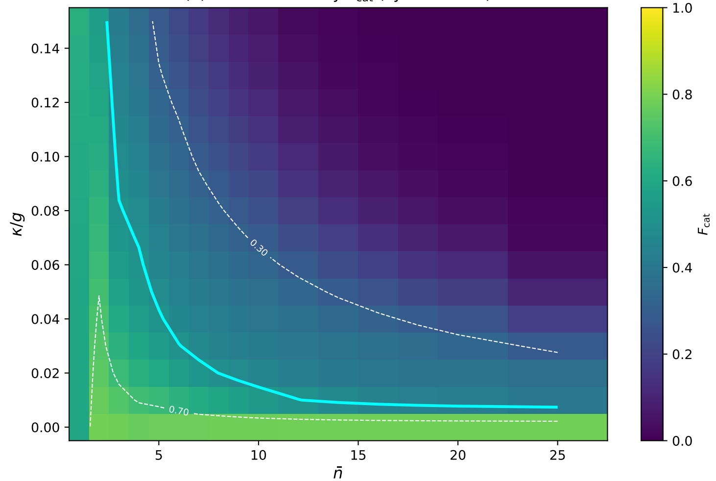
(b) Cat-state fidelity F_{\text{cat}} (cyan: F = 0.5 )
