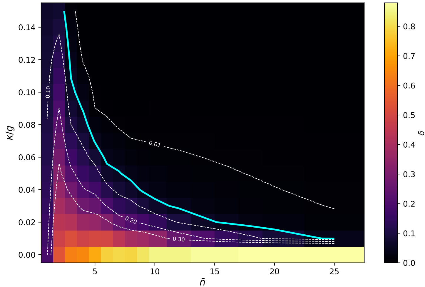
(a) Wigner negativity \delta (cyan: \delta = 0.05 )
