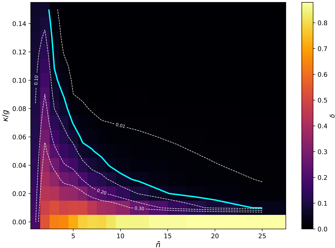
(a) Wigner negativity \delta at t = t_r/2 (cyan: \delta = 0.05 )
