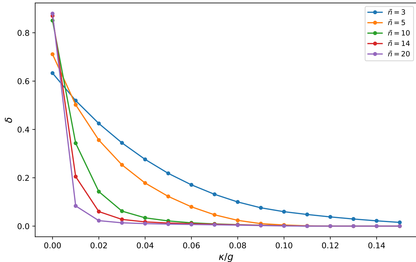
Wigner negativity vs \kappa/g (fixed \bar{n} )
