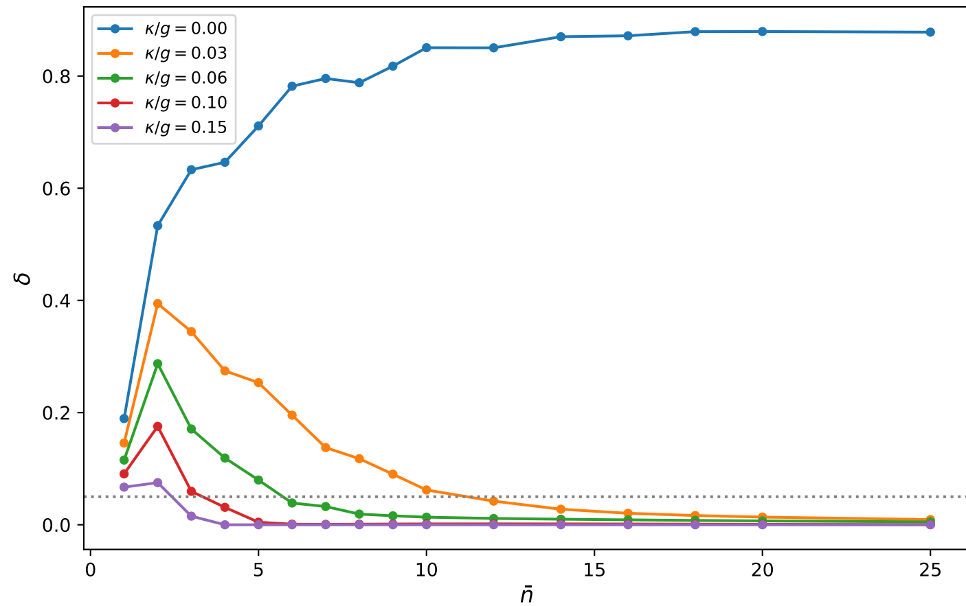
Wigner negativity vs \bar{n} (fixed \kappa/g )
