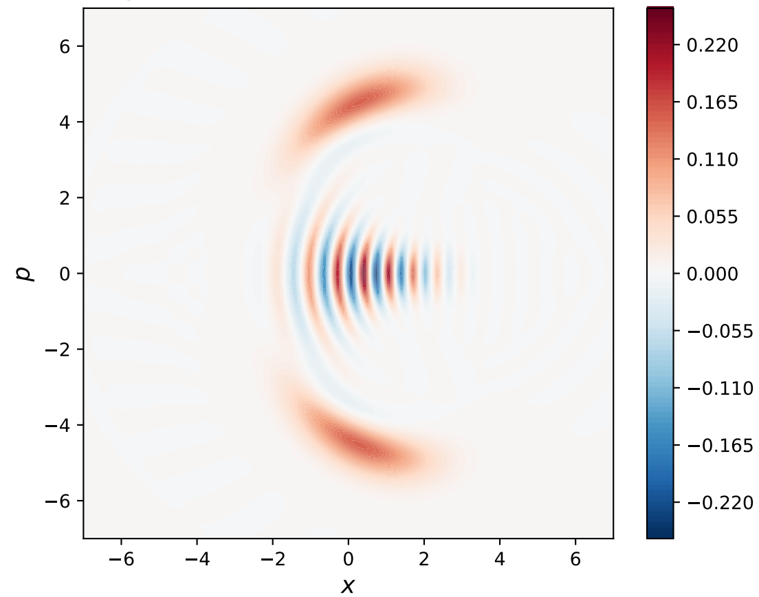
Wigner function at t = t_r/2 (cat state), \delta = 0.85
