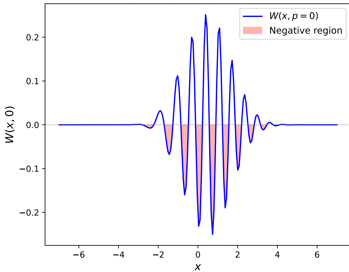
Cross-section at p = 0 : negative regions witness non-classicality
