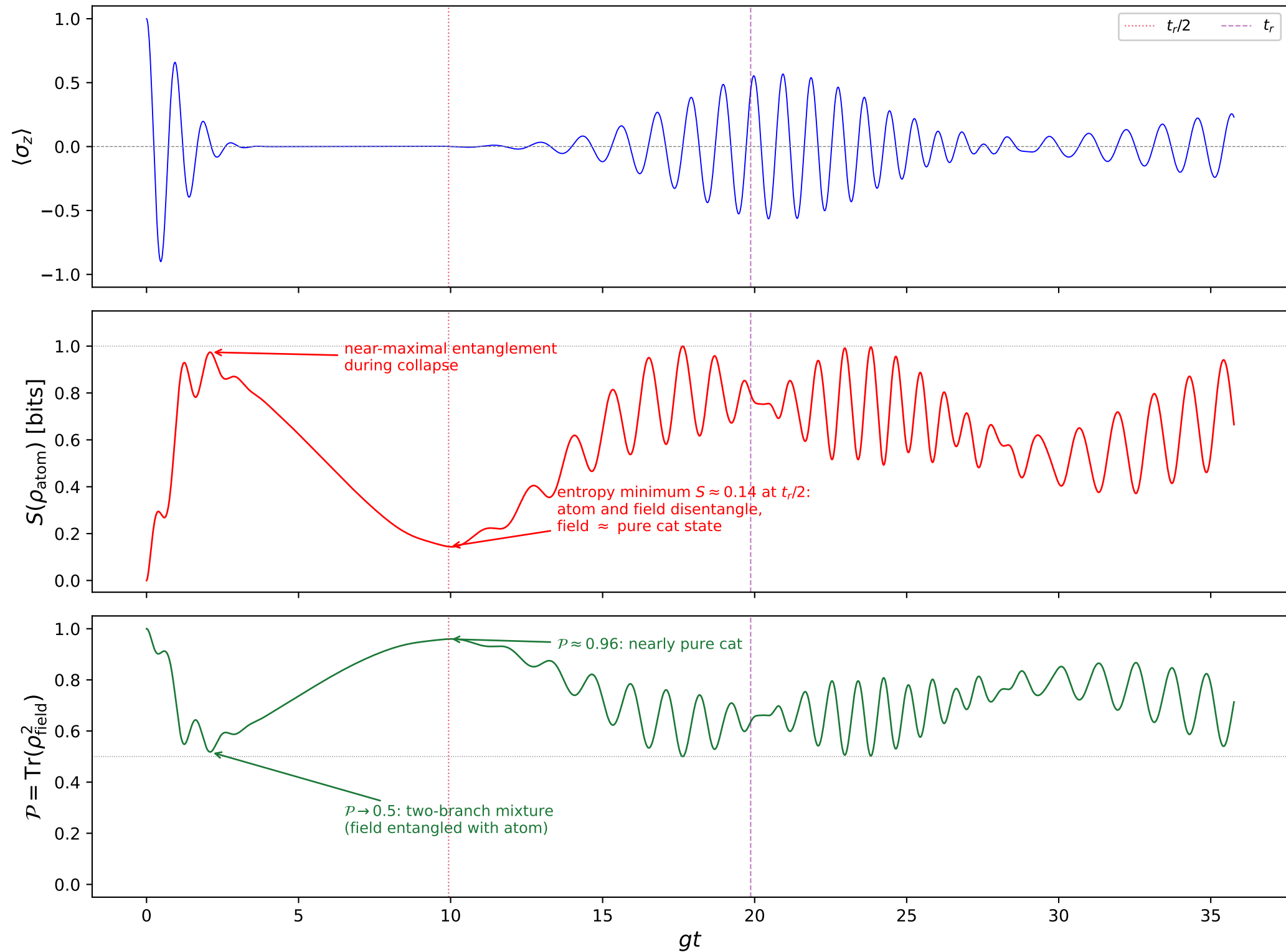
Coherent-state field ( \alpha = 3.16 , \bar{n} = 10 )
