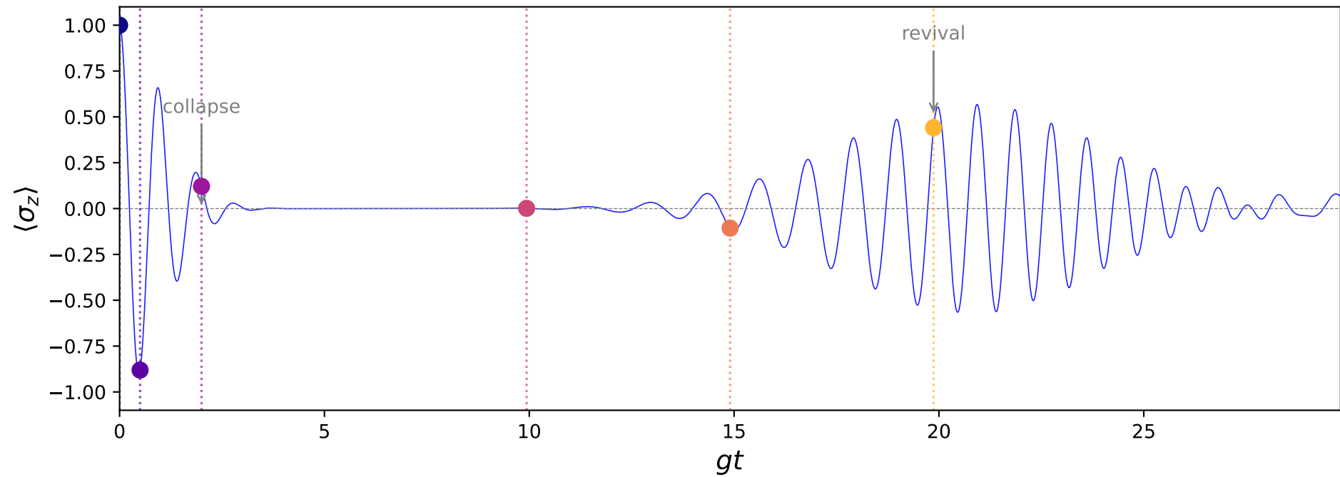
Atomic Inversion ( \bar{n} = 10, \Delta = 0 )
