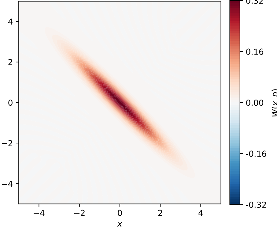
Squeezed vacuum ( r=1, \phi=\pi/2 )
