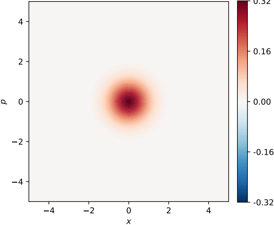
Fock |0\rangle (vacuum)
