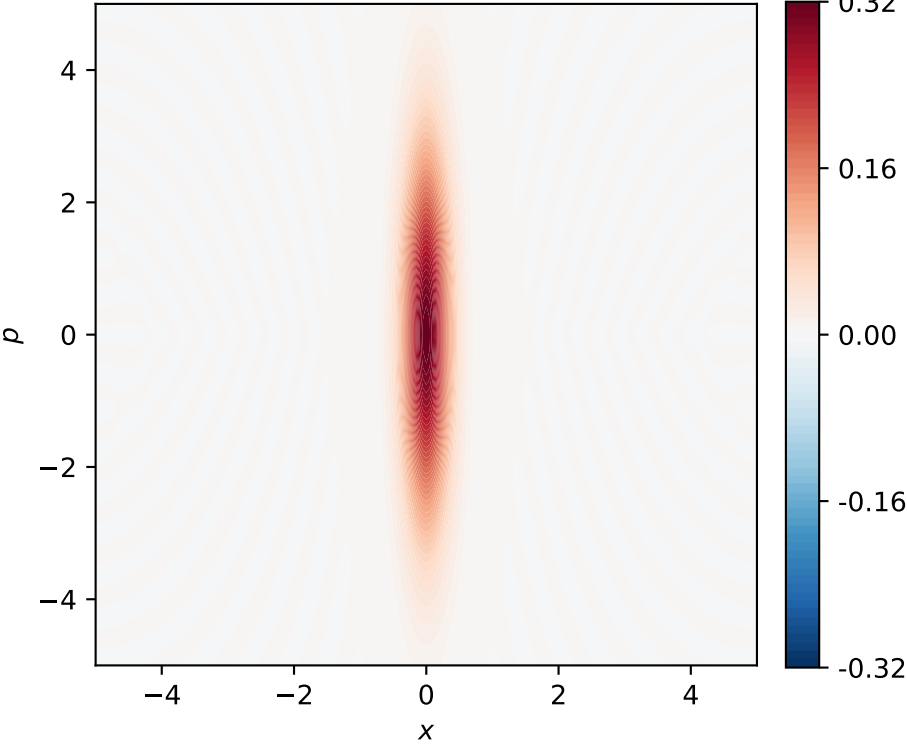
Squeezed vacuum ( r=1, \phi=0 )
