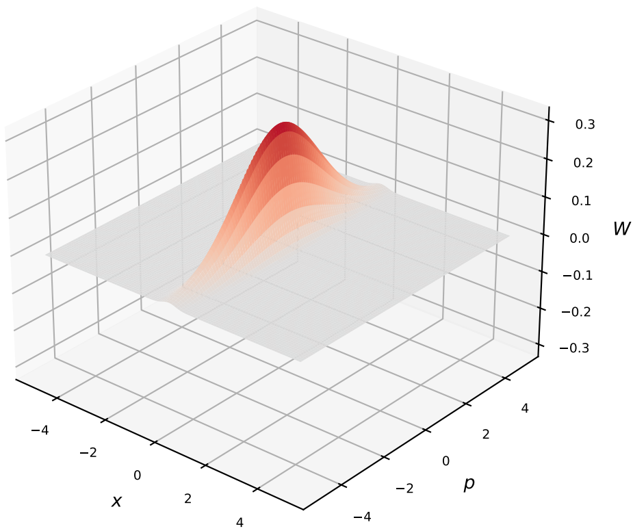
Coherent |\alpha = 2\rangle (no negativity)
