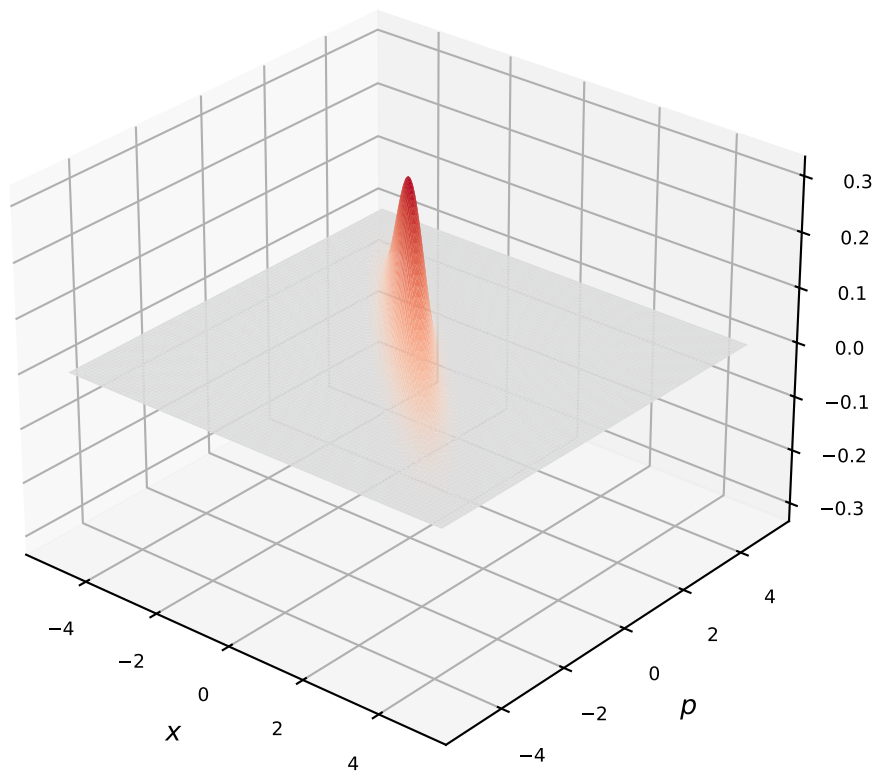
Coherent |\alpha = 2 + 2i\rangle (no negativity)
