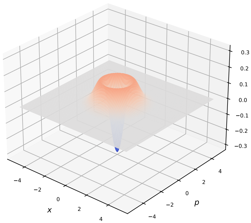
Fock |7\rangle ( W_{\min} = -0.32 )
