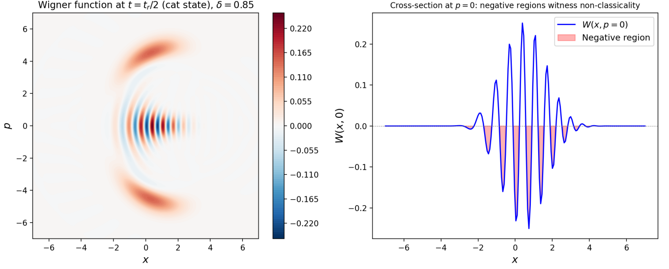
FIG. 3. Detailed view of the Schrödinger cat state formed at t = t_r/2 . Left: Wigner function contour plot showing two coherent-state lobes and interference fringes. Right: cross-section W(x, p = 0) with negative regions (shaded red) reaching W \approx -0.25 ; the fringe spacing is \pi/\sqrt{2\bar{n}} \approx 0.70 . The negativity ( \delta = 0.85 ) confirms the non-classical character of this dynamically generated state, whose fidelity with the best-fitting two-component cat is 0.78.
