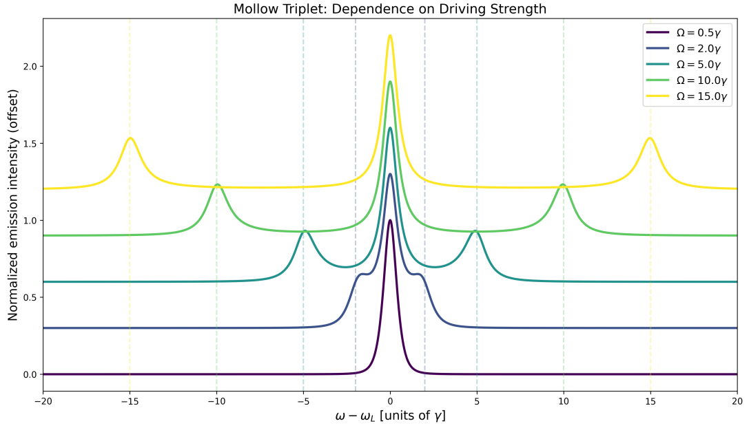
FIG. 12. Mollow triplet spectra for a driven two-level system at varying Rabi frequencies \Omega/\gamma = 0.5 – 15 . As the driving strength increases, the single peak splits into three: a central Rayleigh line and two sidebands at \omega - \omega_L = \pm\Omega .
