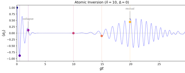
FIG. 1. Atomic inversion \langle \sigma_z(t) \rangle for a two-level atom interacting with a coherent-state field ( \bar{n} = 10 ) in the resonant Jaynes–Cummings model. Colored markers indicate the six snapshot times used for the Wigner function evolution in Fig. 2. The collapse of oscillations near t \approx 2/g and the first revival at t_r \approx 19.9/g are clearly visible.
