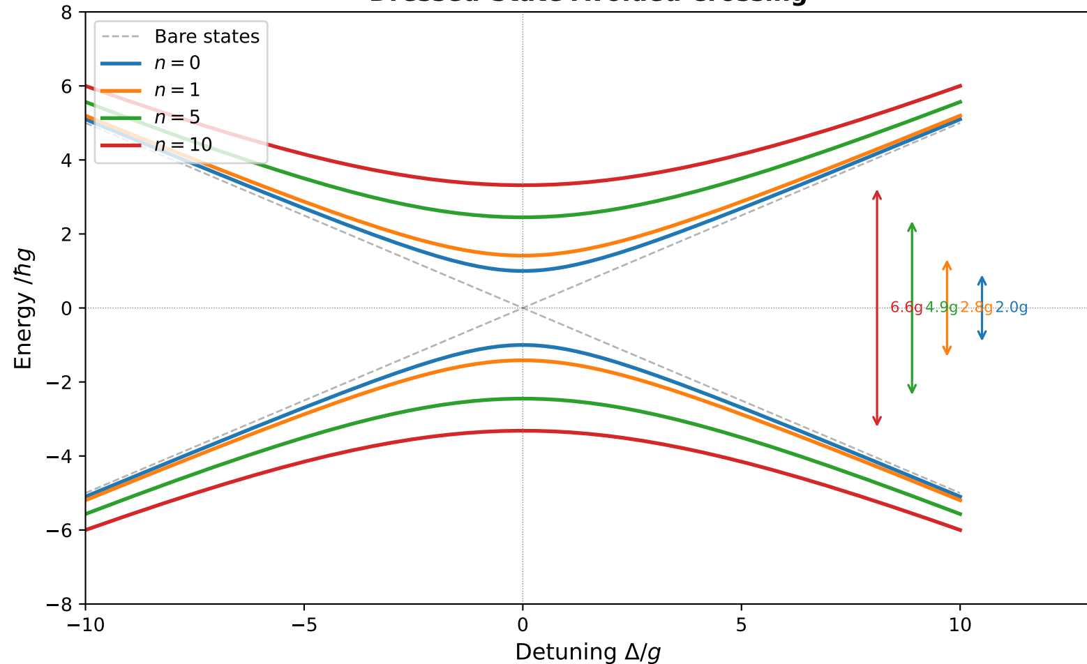
Dressed-State Avoided Crossing
