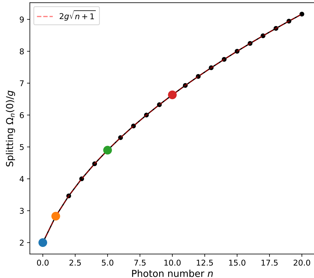
\sqrt{n+1} Scaling at \Delta = 0
