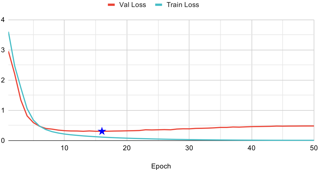
CTC Loss in Validation and Train vs. Epochs
