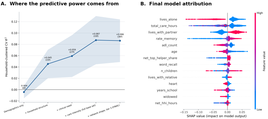
HRS 2022, n = 2,142 . Panel A adds feature blocks cumulatively under identical five-fold GroupKFold folds; the shaded band is one standard deviation across folds and is wide enough that the last two steps overlap, so the apparent gain from network structure is not distinguishable from noise. Panel B: each dot is one respondent, horizontal position is that feature's contribution to their prediction, and color is the feature value. Network-structure features receive 6% of total SHAP attribution, so they are real but clearly secondary to living arrangement and care intensity.
