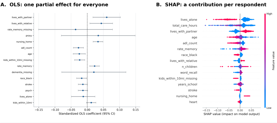
Panel A: standardized OLS coefficients, so 0.06 means a one-standard-deviation increase is associated with a 6-percentage-point higher informal share, holding every other predictor fixed; bars are 95% confidence intervals. Panel B: each dot is one held-out respondent, horizontal position is how far that feature moved that person's prediction away from the average, and color is the feature value, red high and blue low. A coefficient and a mean absolute SHAP value are not the same quantity, which is why the rankings diverge. The two features that move furthest between the rankings are lives_alone , which is first by SHAP and 24th by coefficient because the living-arrangement indicators are nearly collinear, and total_care_hours , whose relationship to the outcome is non-monotone.
