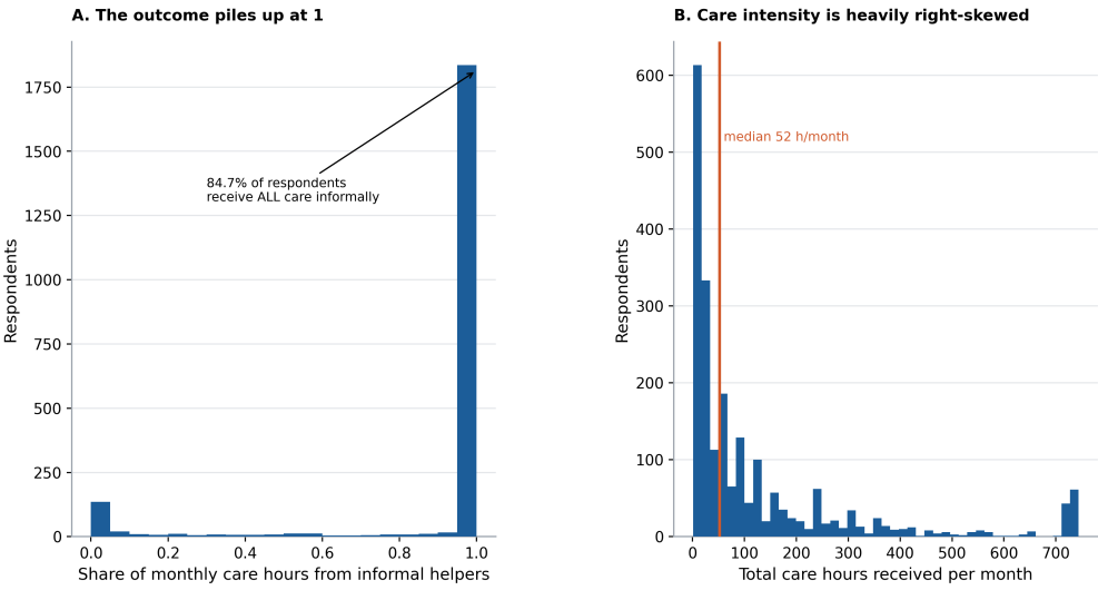
HRS 2022, n = 2,142 respondents receiving any help with ADLs or IADLs. Panel A: informal share = informal care hours / total care hours per month. Panel B is truncated at the physical ceiling of 24 hours \times 31 days. The mass at 1.0 in Panel A is why a plain linear model is a poor match and why script 03 fits a two-part specification.
