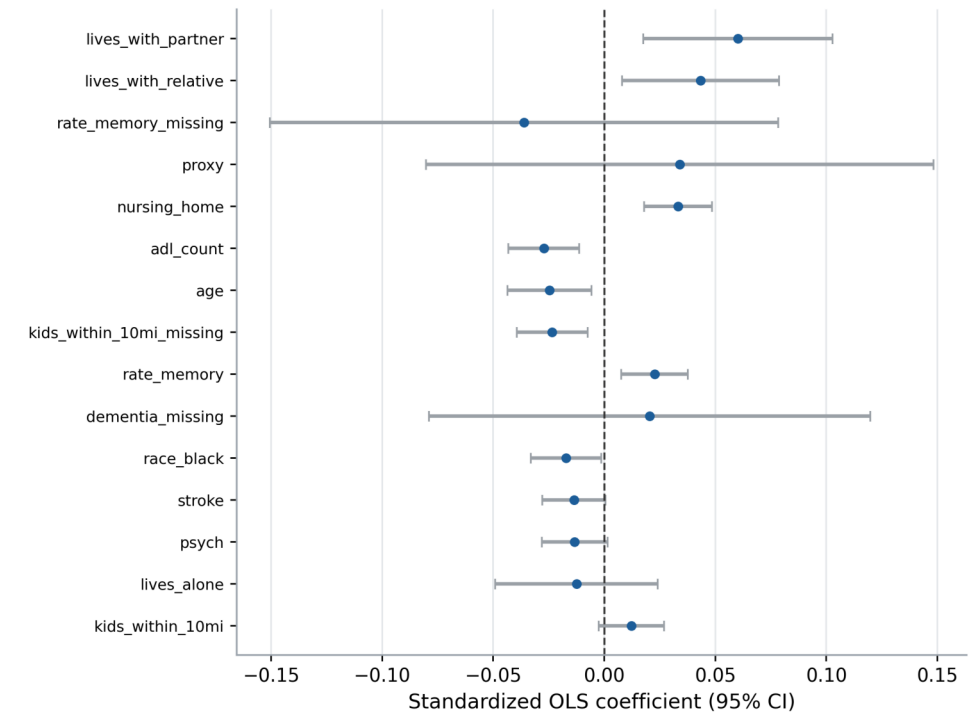
A. OLS: one partial effect for everyone
